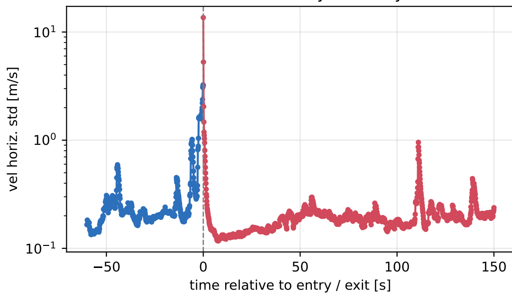
Horizontal velocity accuracy
