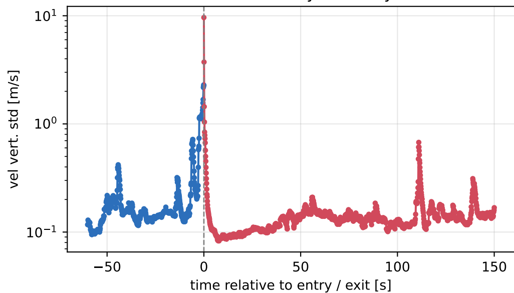
Vertical velocity accuracy
