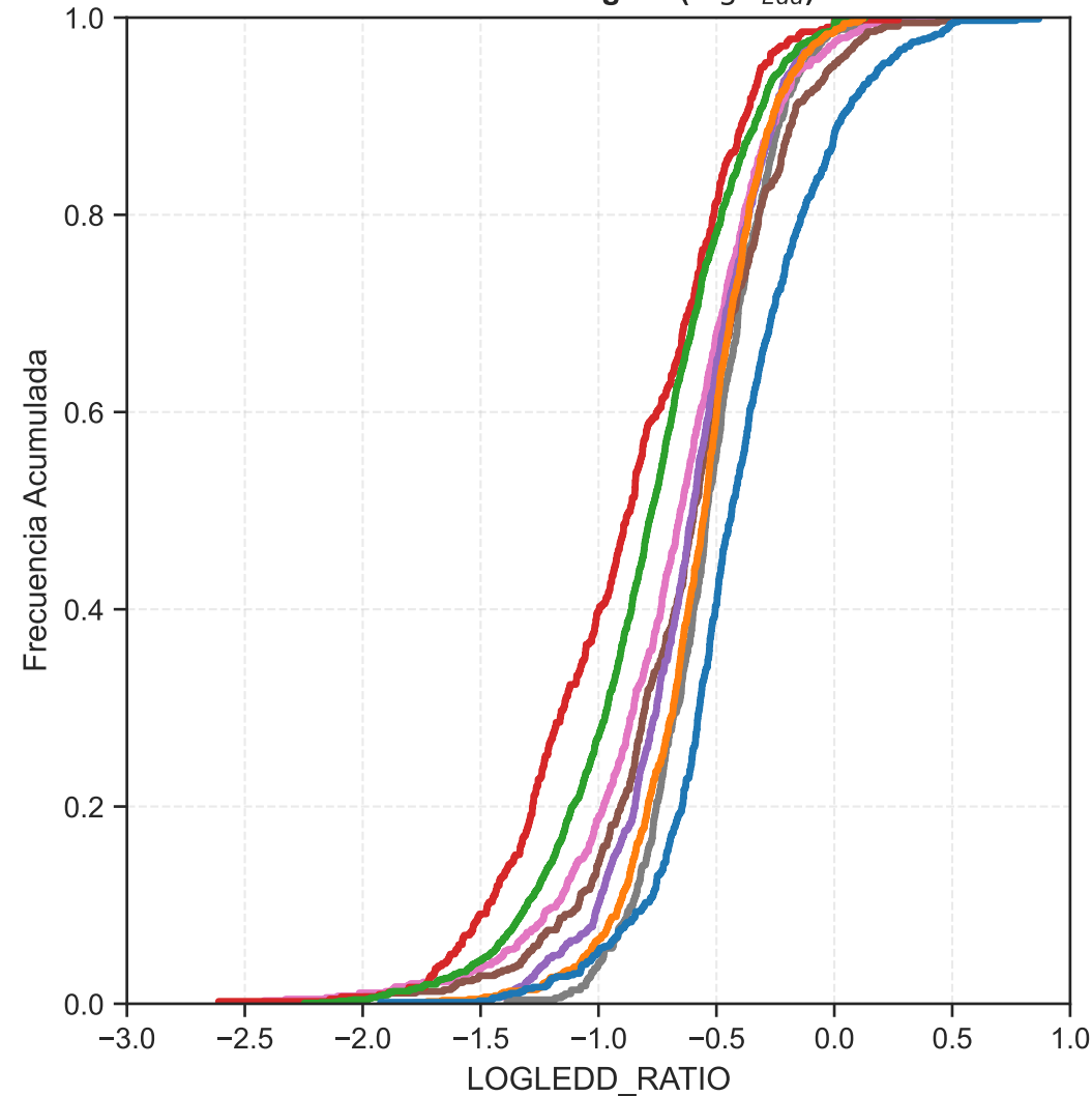
Ratio de Eddington ( \log \lambda_{Edd} )
