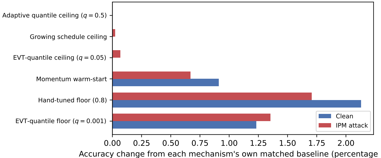
Six clipping/momentum mechanisms vs. their own matched baselines (none reaches significance; see Table 1)
