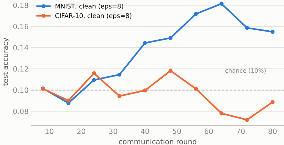
Convergence trace, seed 0, T=80
