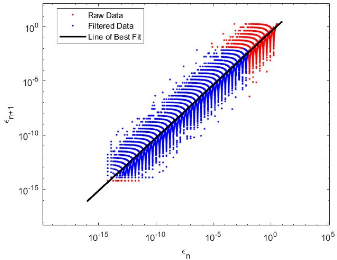
Bisection Method Error
