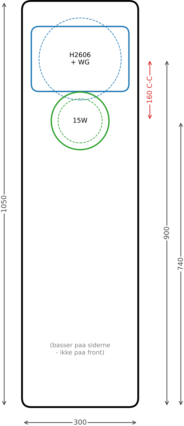
FRONT
