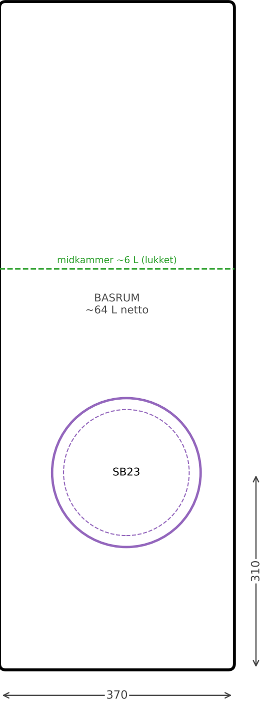
SIDE
