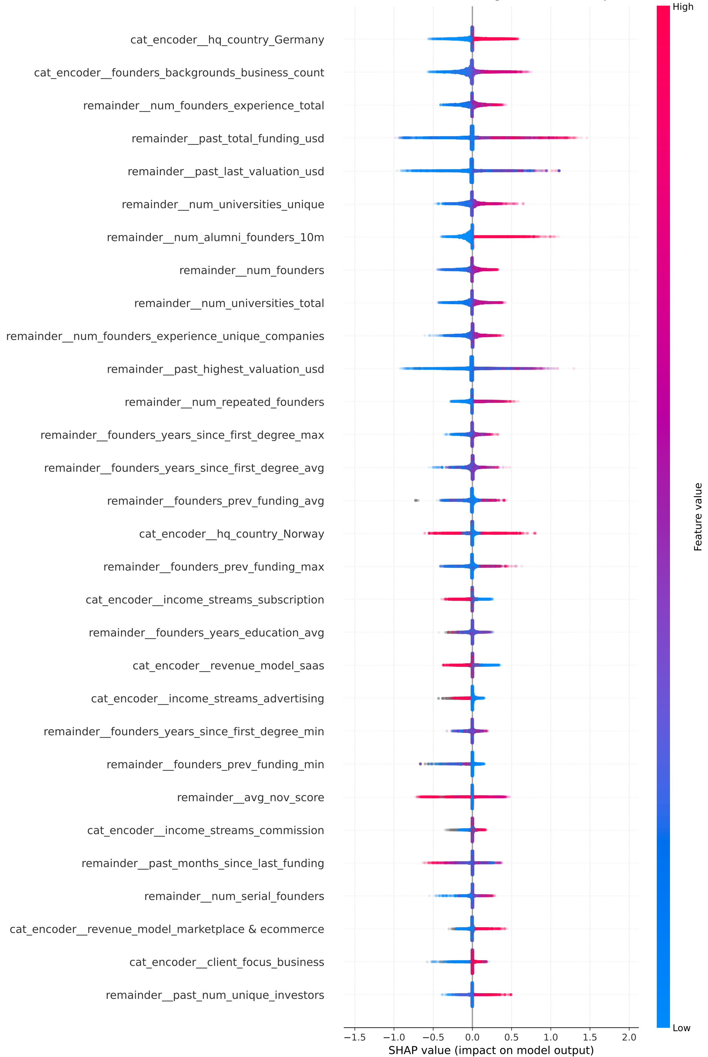
SHAP Beeswarm - All Targets Combined (Top 30)
