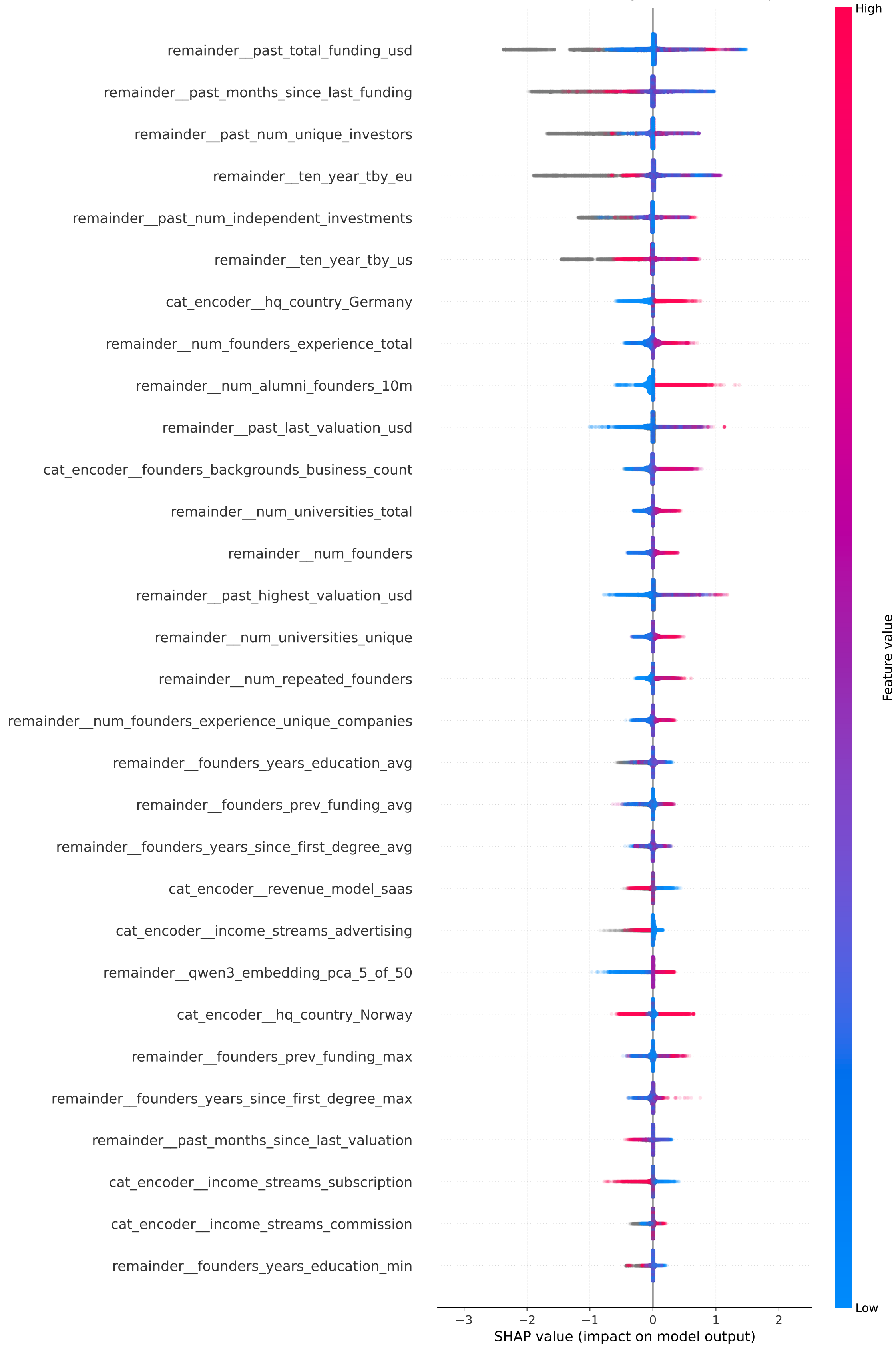
SHAP Beeswarm – All Targets Combined (Top 30)
