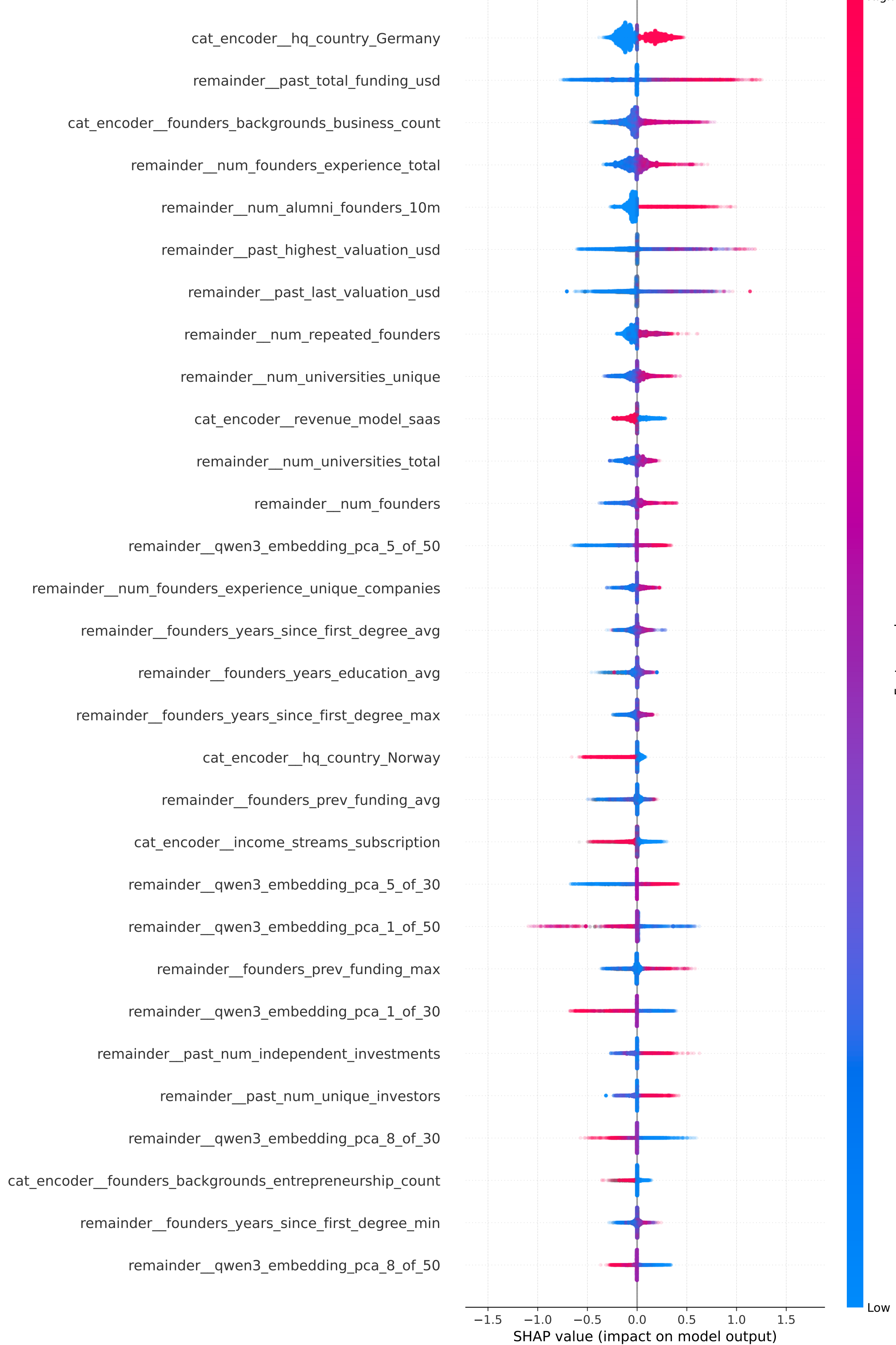
SHAP Beeswarm - target_funding_delta_upper_q
