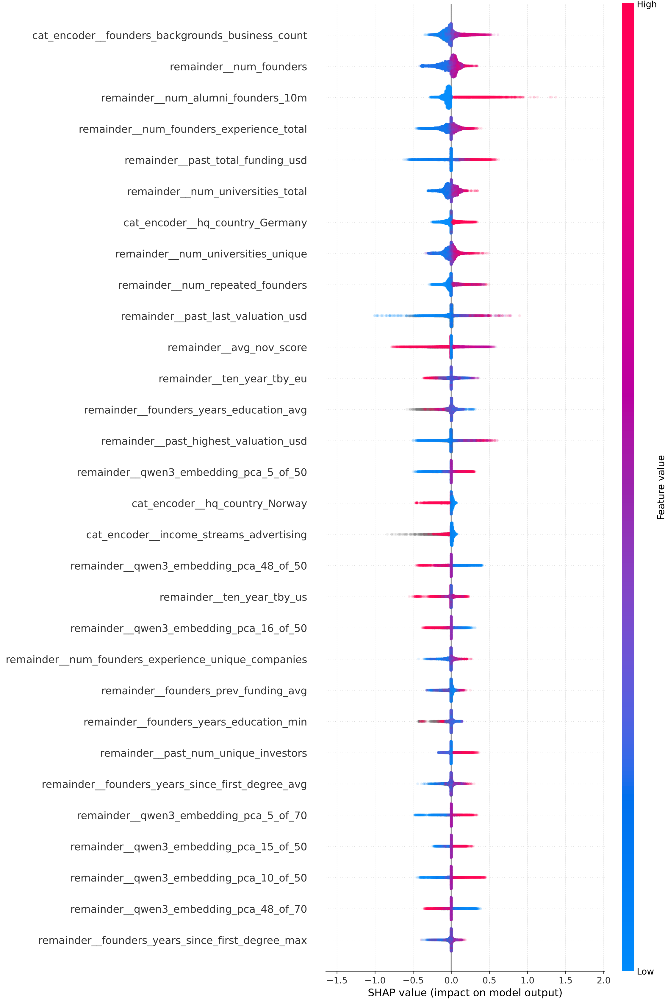
SHAP Beeswarm - target_employee_delta_upper_q
