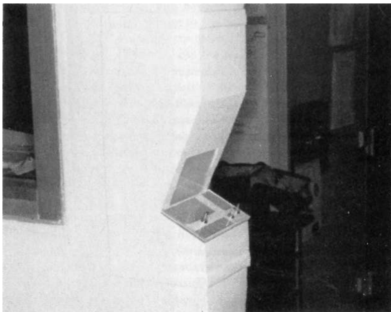
4.8 The original layout of switches in my laboratory had the light switches scattered. We put all the switches in one convenient location, arranged on a floor plan of the laboratory. (The switch panel was constructed by David Wargo.)
