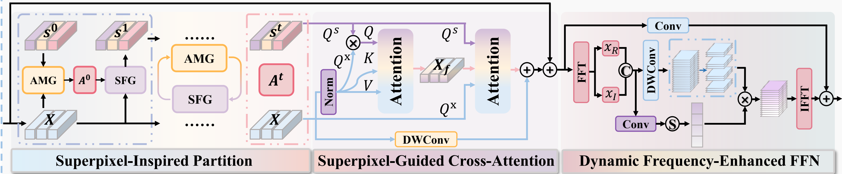
(b) Superpixel-Perceptive Transformer (SPT) Module
