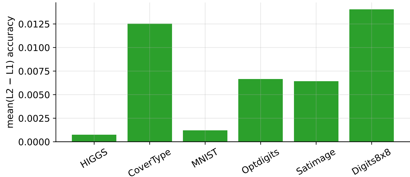
Effect of a second layer by dataset
