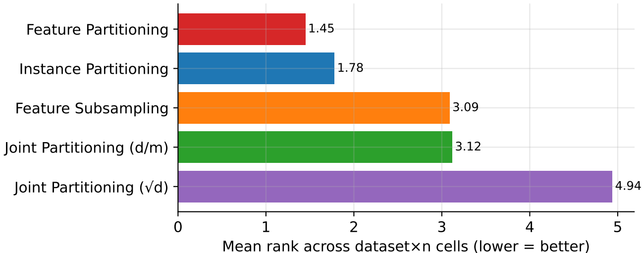
Diversity-strategy ranking at m = 10 (budget-matched arms)
