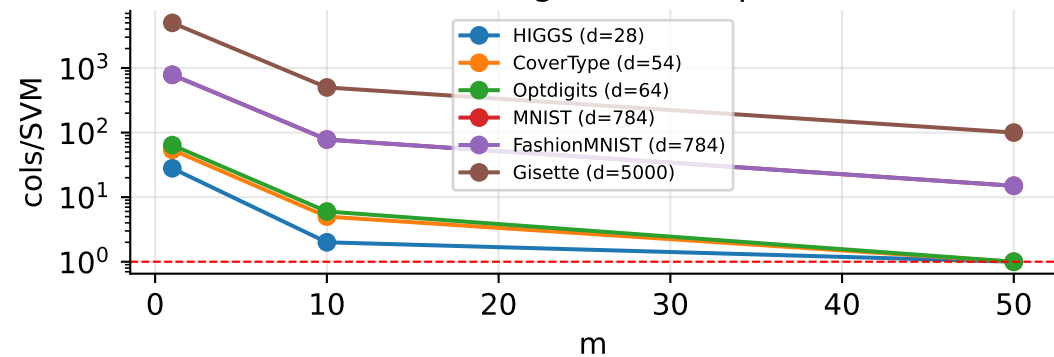
Feature Partitioning: columns per SVM vs m
