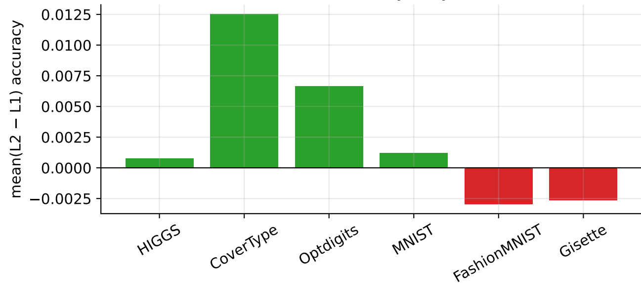
Effect of a second layer by dataset
