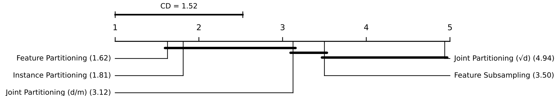
Critical-difference diagram (Nemenyi, \alpha = 0.05 )
