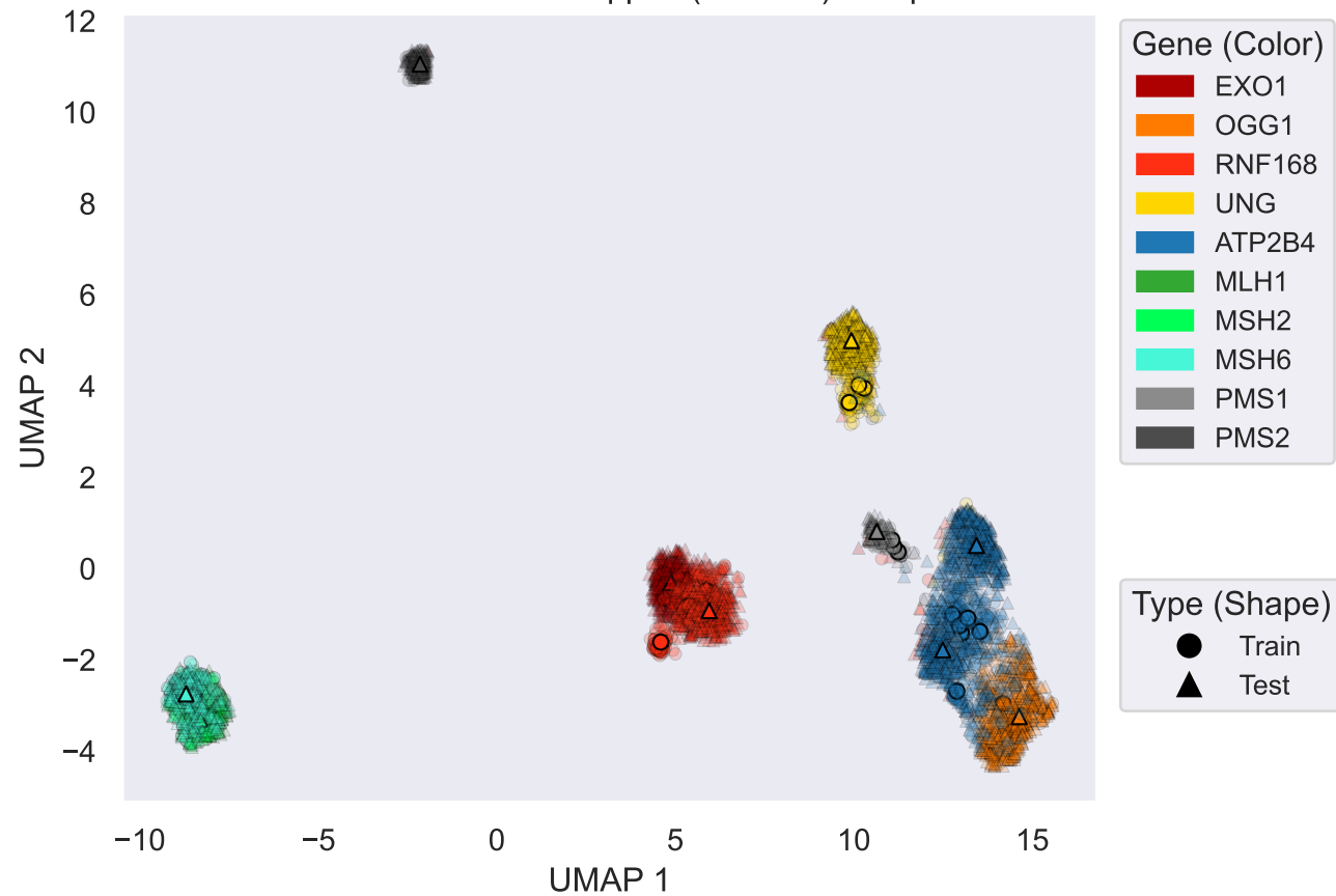
UMAP: Real vs Bootstrapped (Dirichlet) Samples
