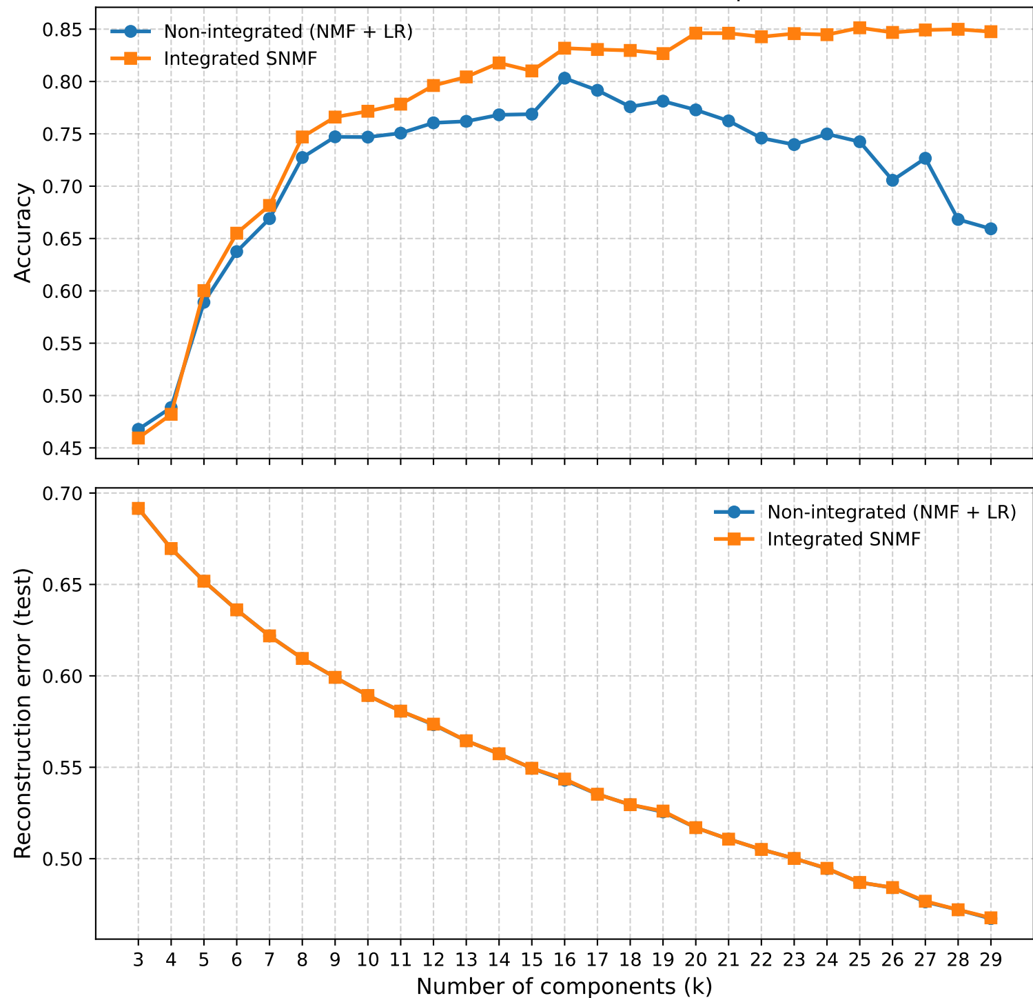
MNIST: Performance vs. Number of Components (k)
