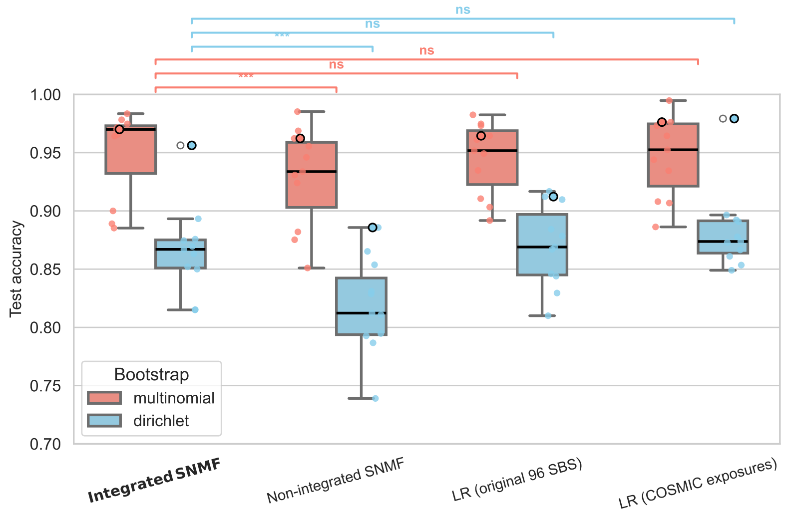
Accuracy by Method and Bootstrap Type
