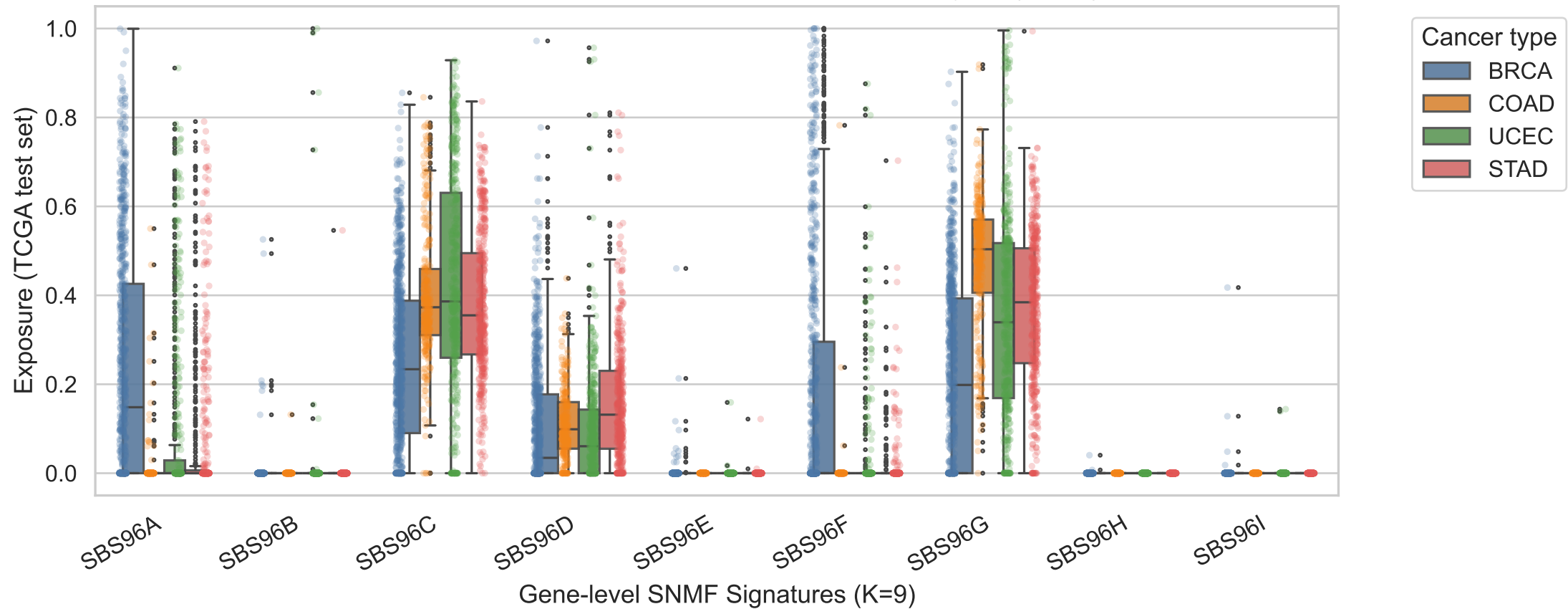
Gene-level SNMF exposure distribution across cancer types (TCGA)
