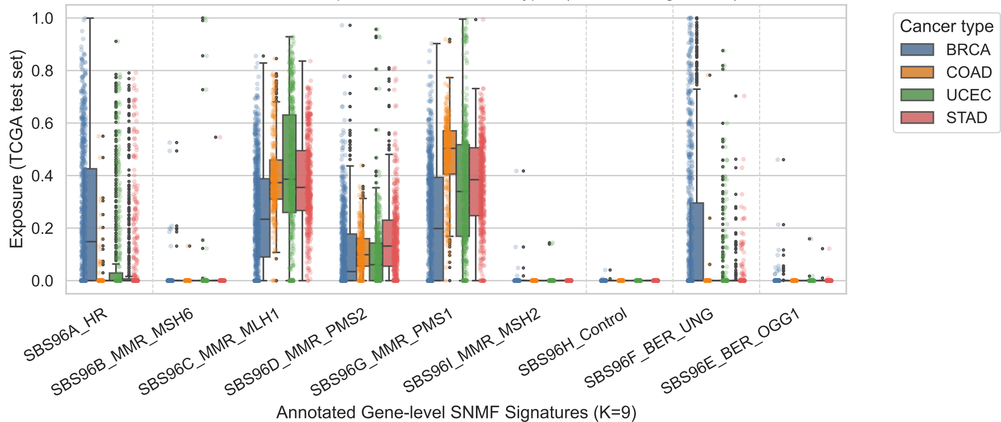
Gene-level SNMF exposures across cancer types (annotated signatures)
