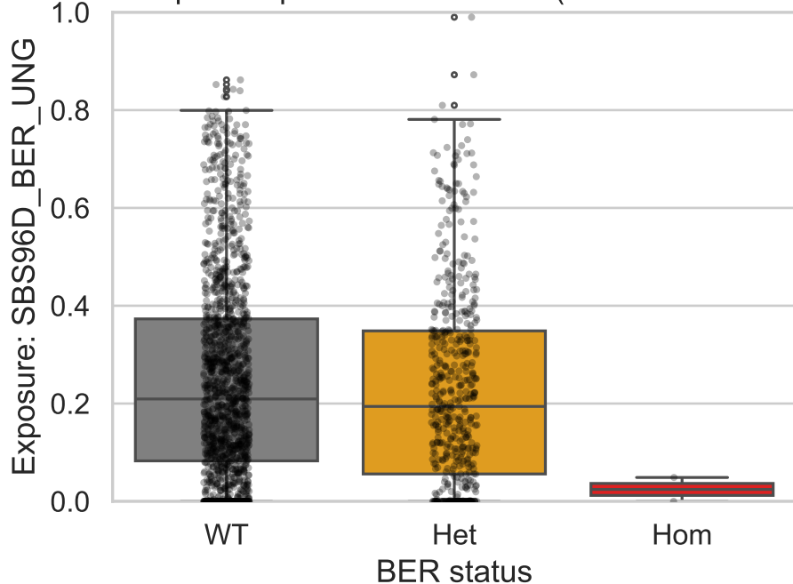
BER-UNG exposure per mutation status (combined HRD + MMRD)
