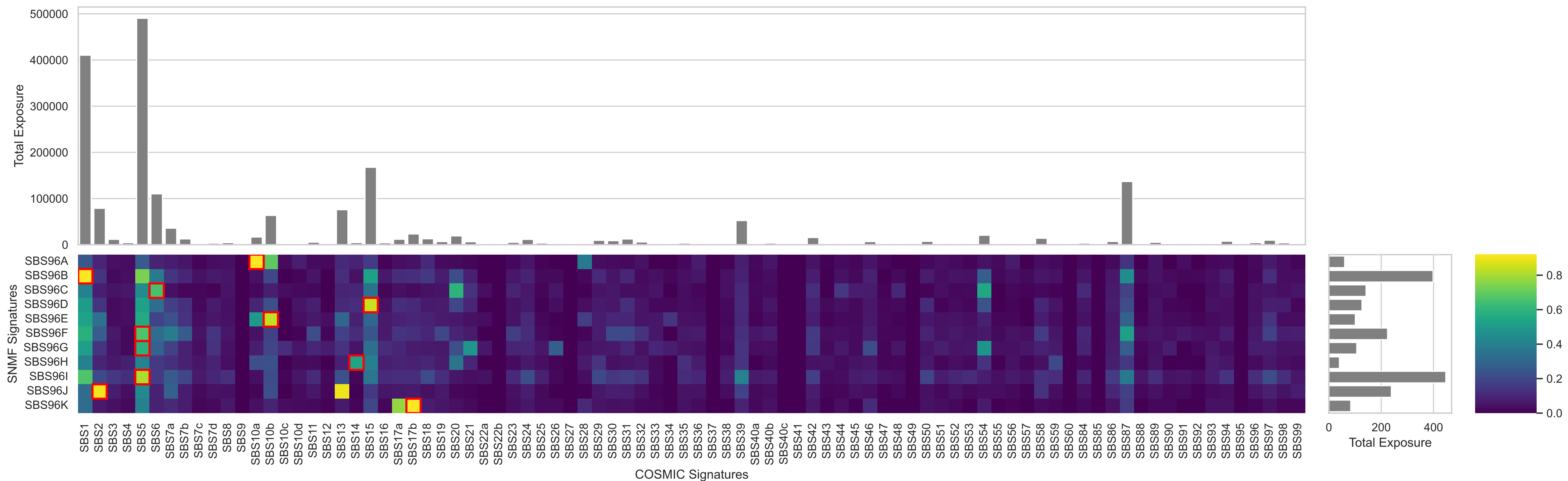
De-novo vs COSMIC Exposure Similarity (Cosine)
