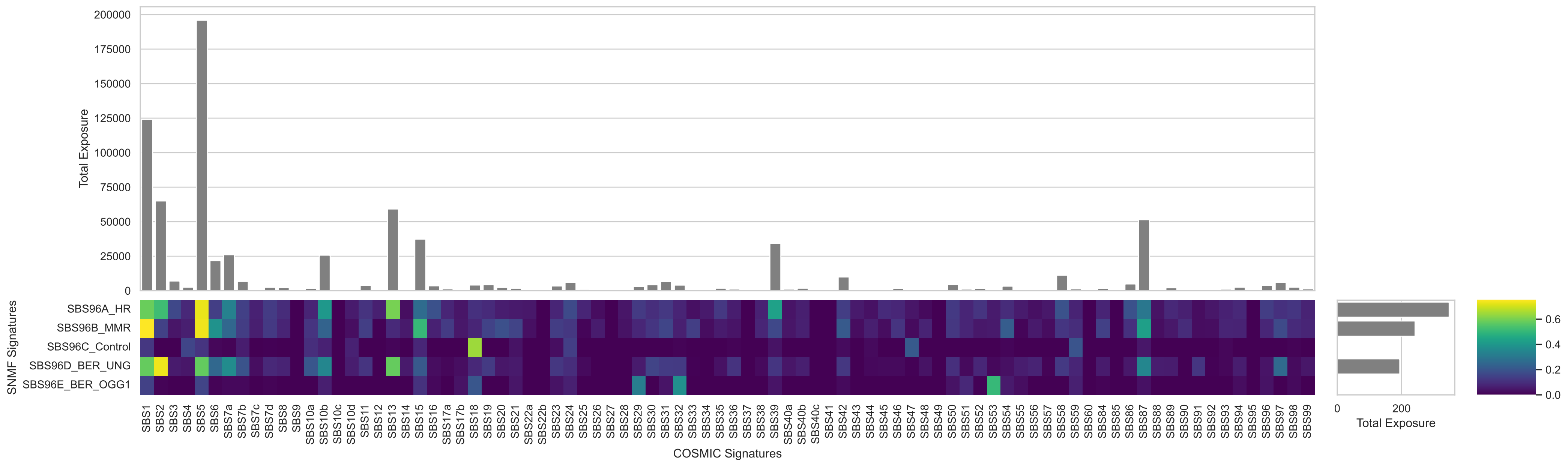
SNMF vs COSMIC Exposure Similarity (Cosine)
