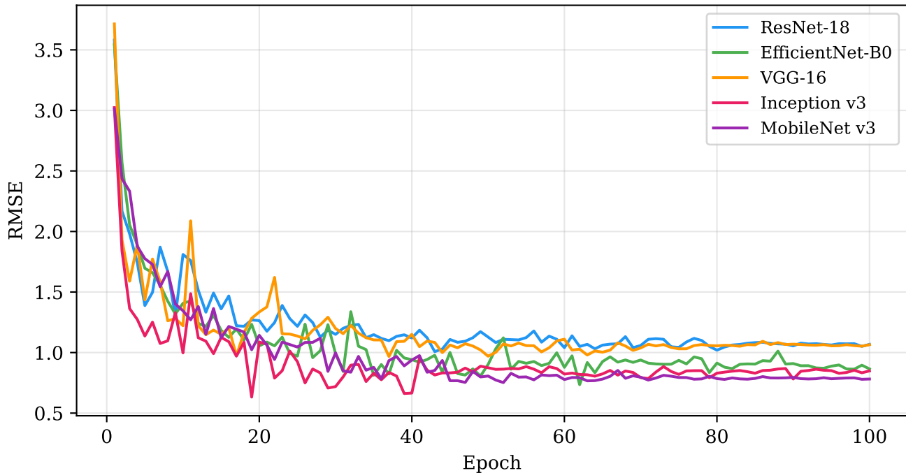
Validation RMSE
