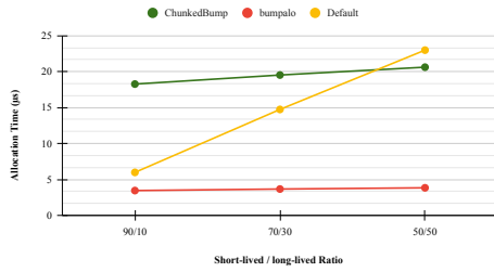
Allocation Time Across Mixed Lifetime Workloads
