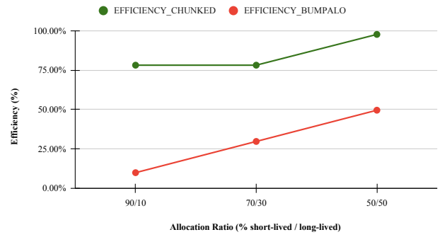
(b) Memory efficiency across allocation ratios
