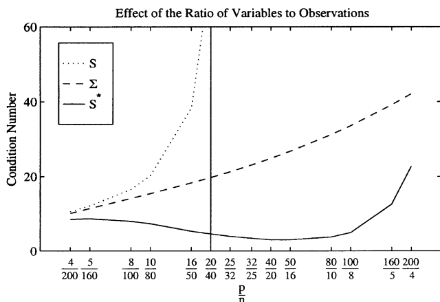
Fig. 9. Effect of the ratio of number of variables to number of observations on the condition number.
