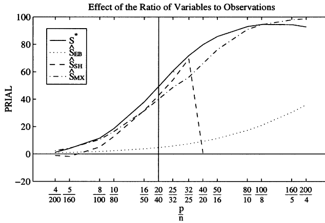
Fig. 6. Effect of the ratio of number of variables to number of observations on the PRIAL: \hat{S}_{SH} is not defined when p/n > 2 because the isotonic regression does not converge.
