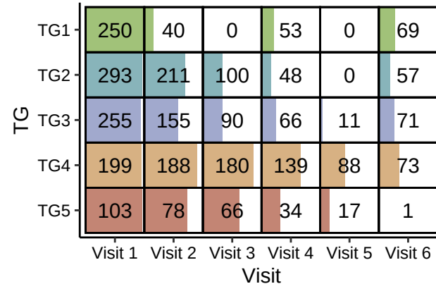
Pbmc Transcriptomics
