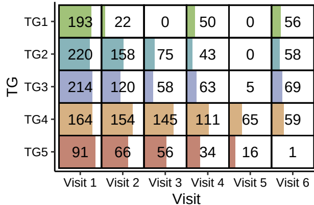
Nasal Transcriptomics
