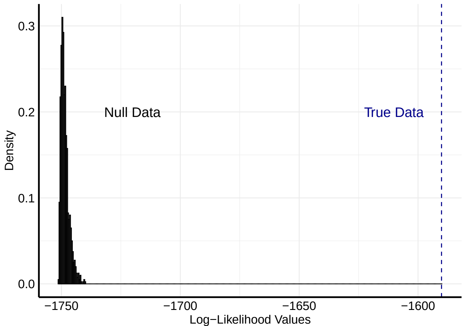
Histogram of Log-Likelihood Values
