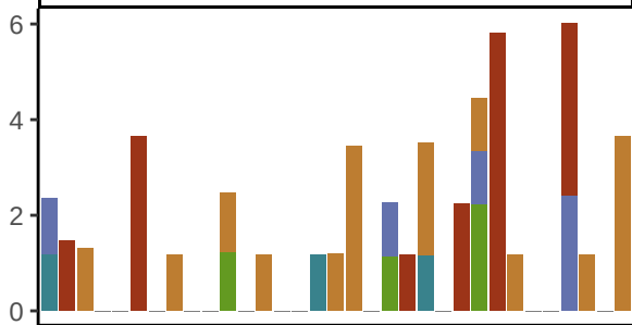
HSV2.nasal
