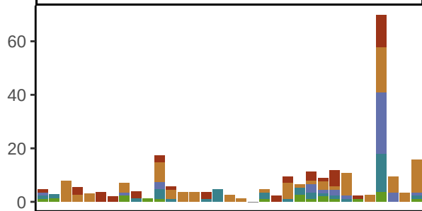
HSV1.nasal
