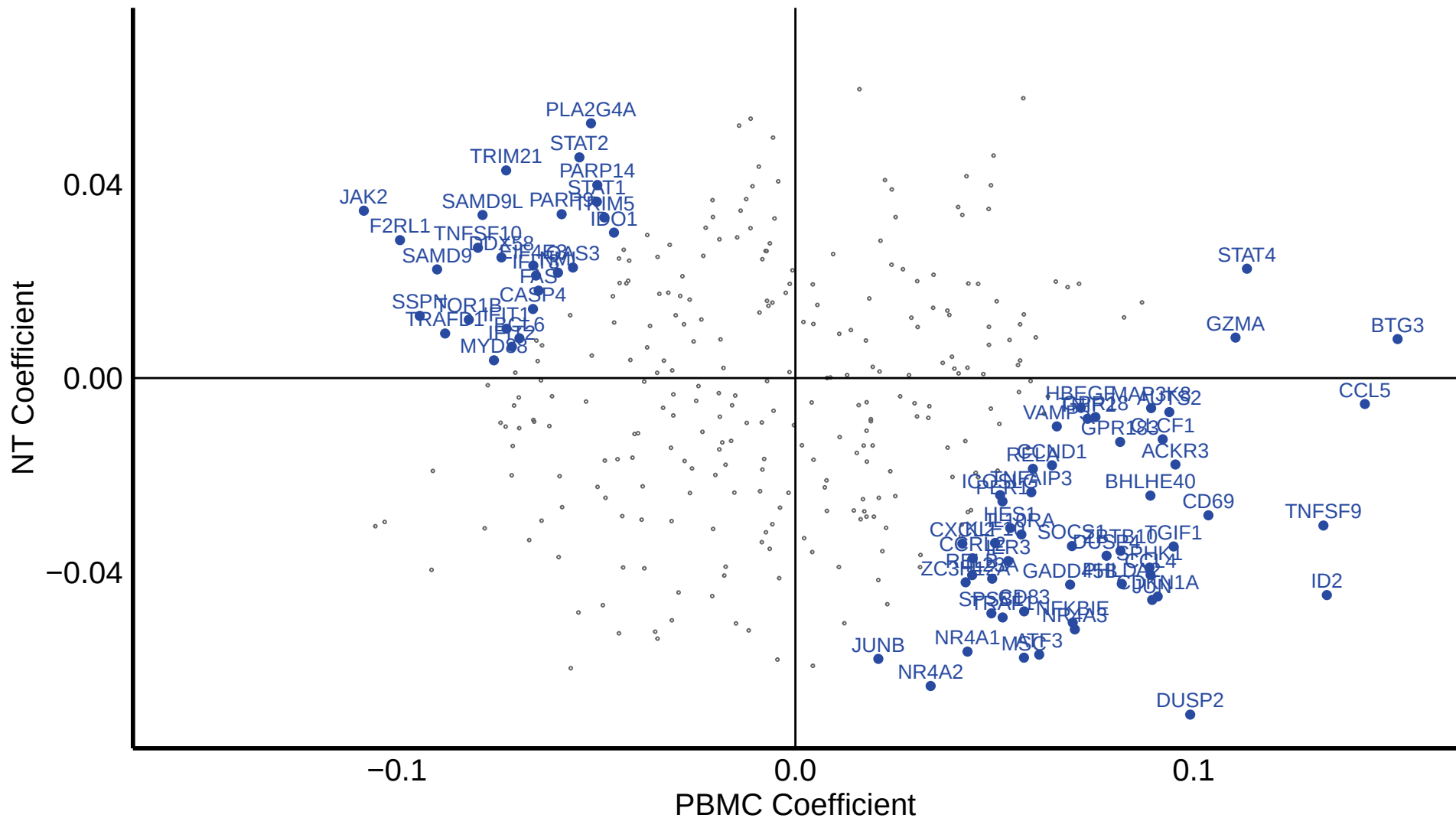
Coefficient Comparison Between PBMC and Nasal Transcriptomics
