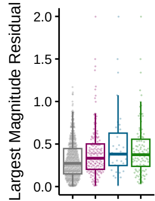
S-methylcys
