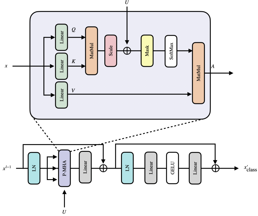
(b) Structure of the particle attention block and the incorporation of the pairwise interaction embedding U .
