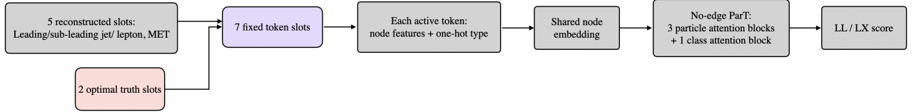
Figure 20: Model structure for oracle tests. Two optimal truth slots are added.
