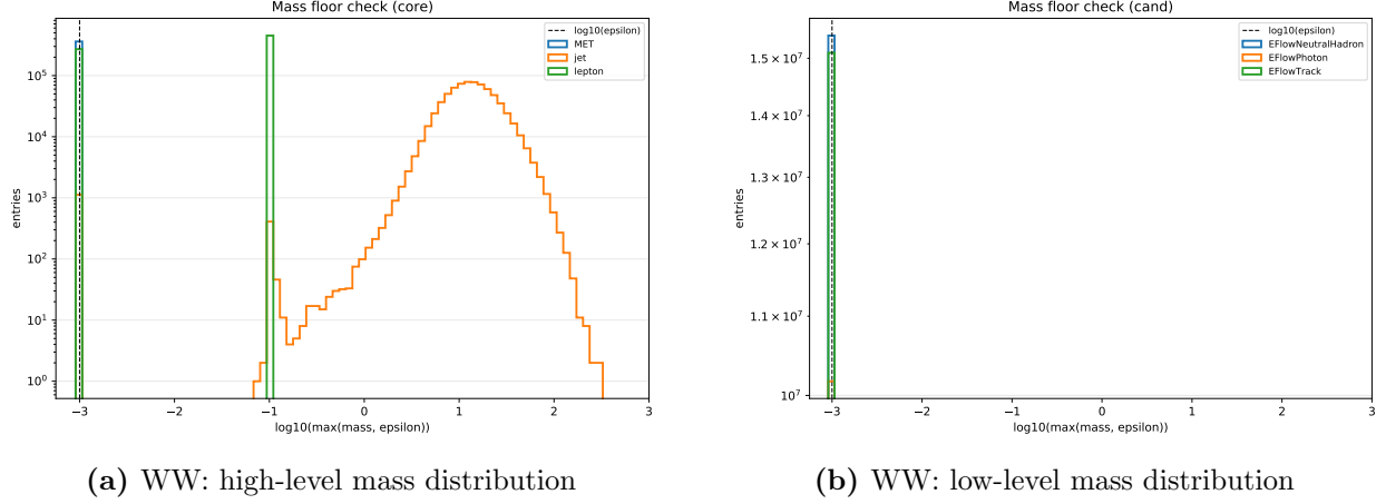
Figure 17: Mass distributions for the WW high-level and low-level tasks.
