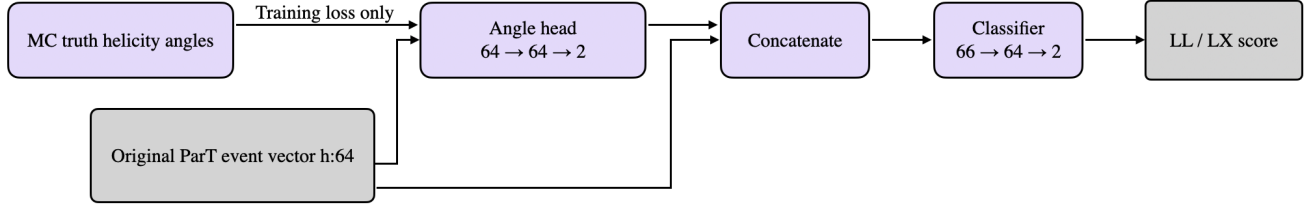
Figure 23: Model structure for helicity angle series testings.
