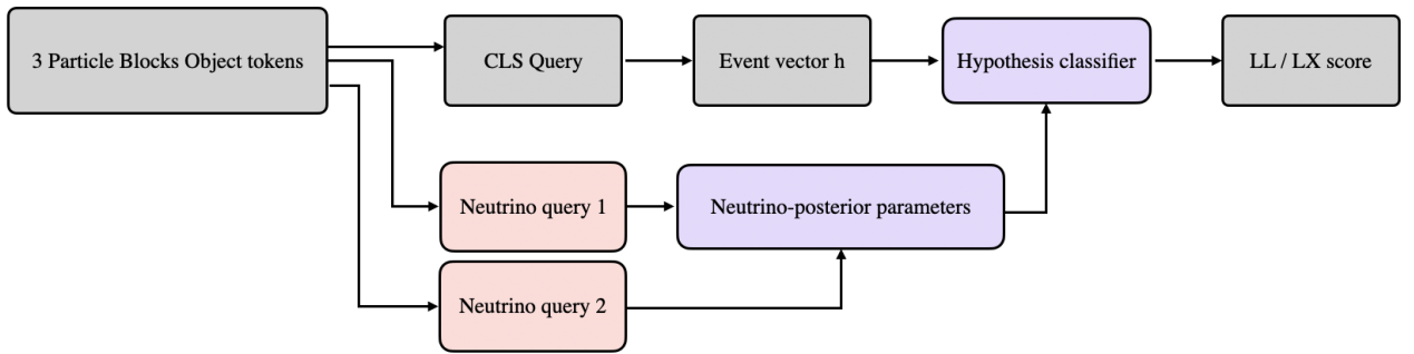
Figure 22: Model structure for the Neutrino Series testings.
