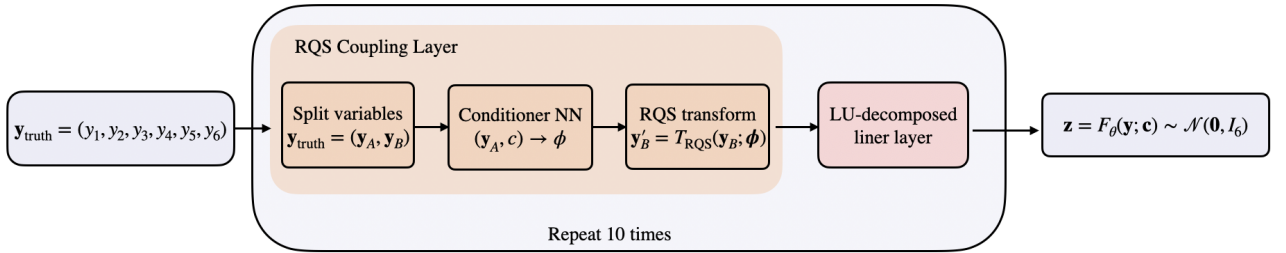
Figure 25: The conditional normalizing flow model structure for \nu^2 Flow
