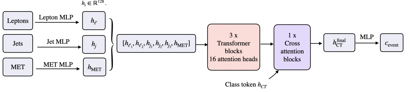
Figure 24: The event encoder model structure for \nu^2 Flow
