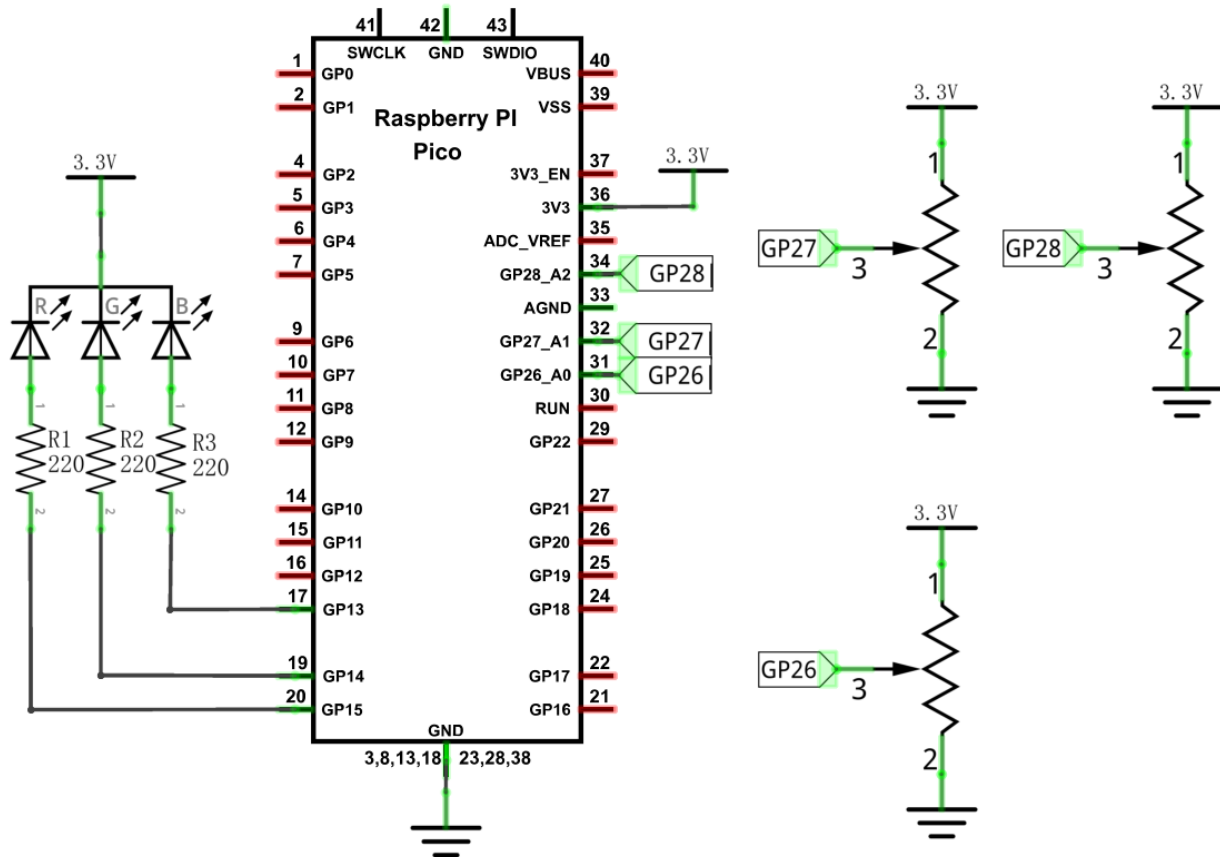
Schematic diagram
