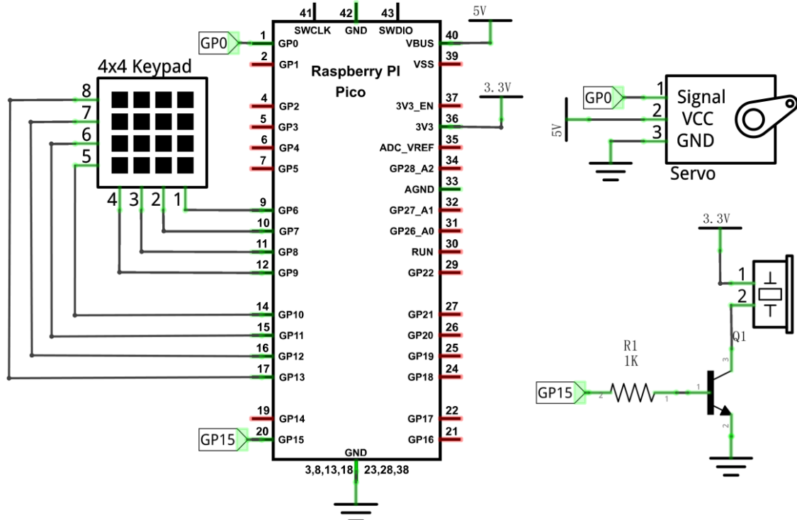
Schematic diagram
