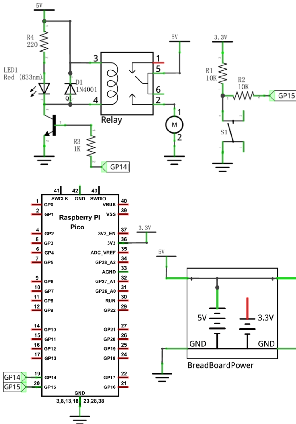
Schematic diagram
