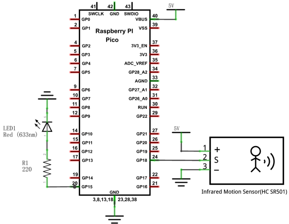
Schematic diagram
