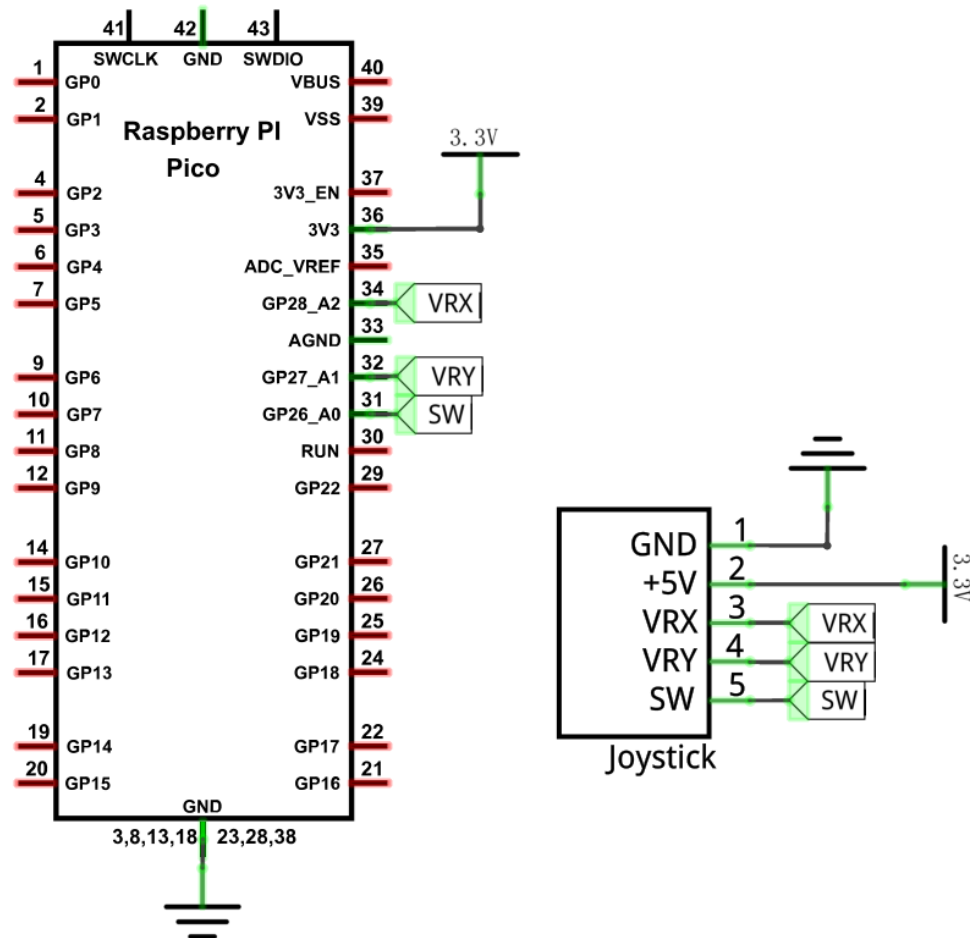
Schematic diagram
