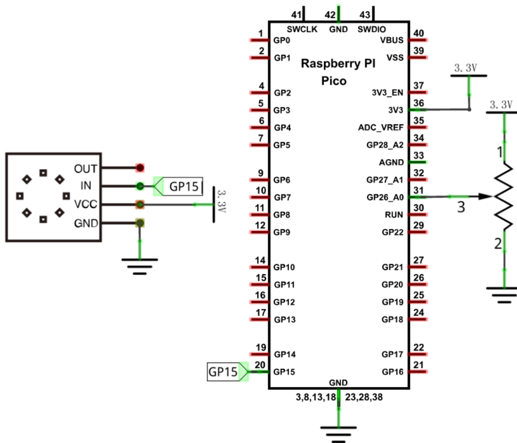
Schematic diagram
