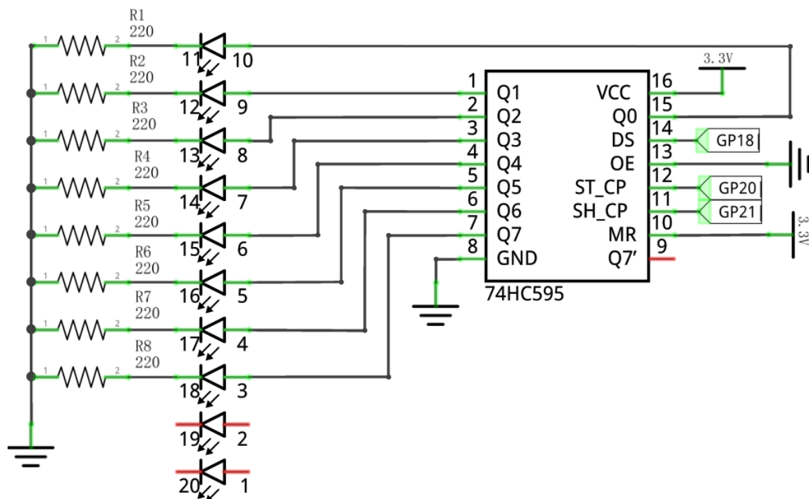
Schematic diagram
