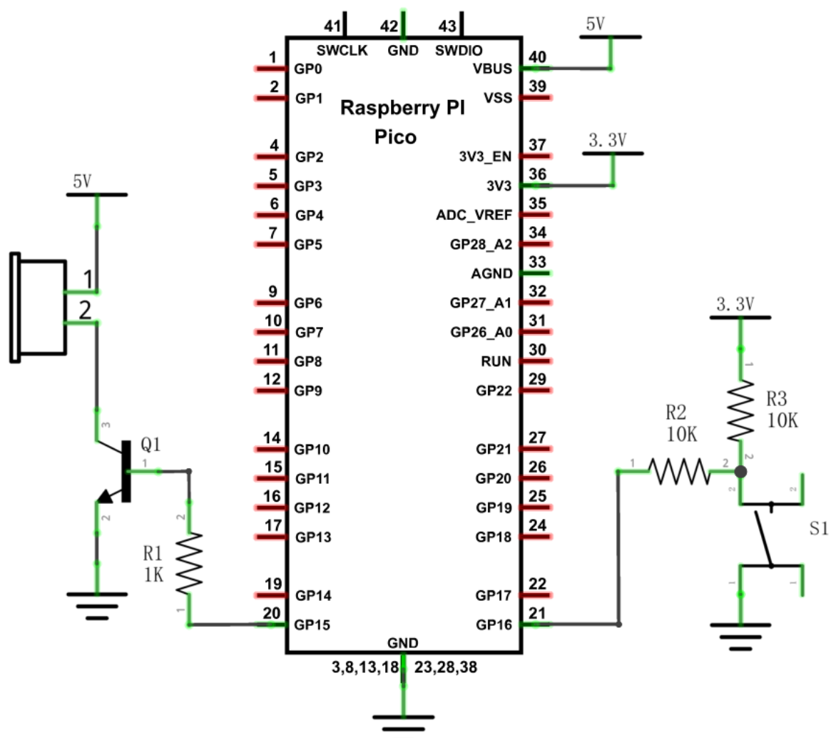
Schematic diagram
