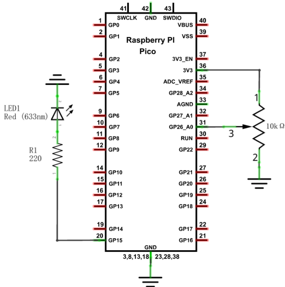
Schematic diagram
