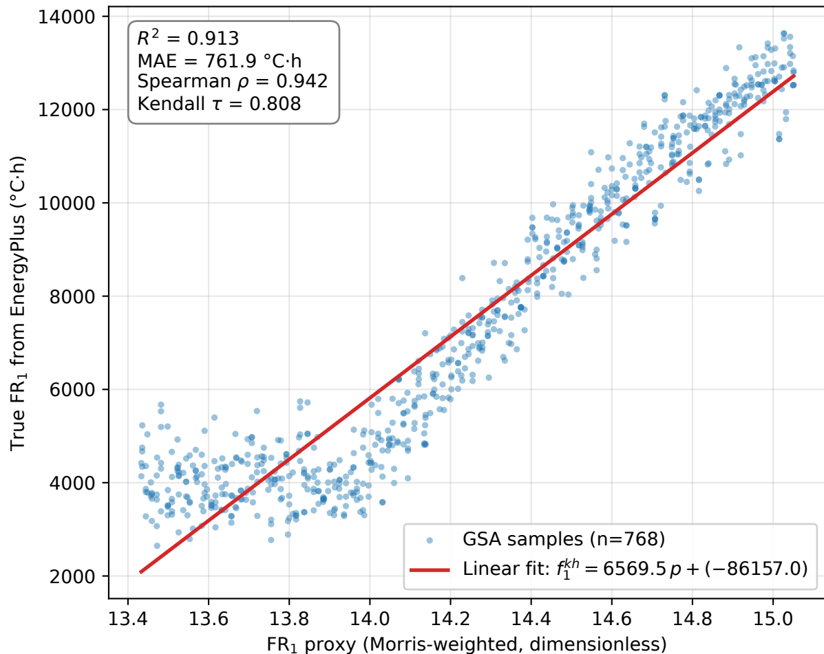
FR 1 proxy calibration vs. EnergyPlus ground truth
