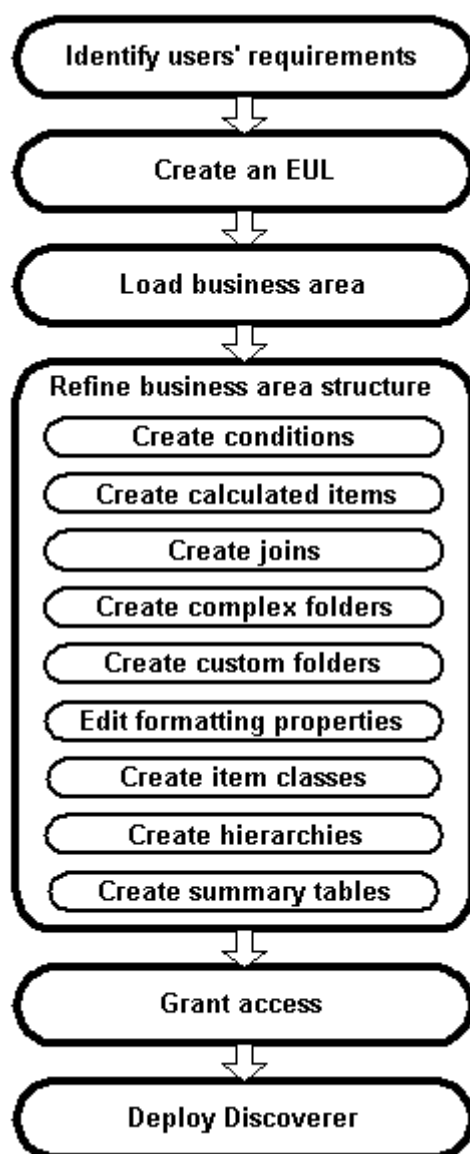
Description of "Figure 3-2 Discoverer implementation flowchart (with a relational data source)"
