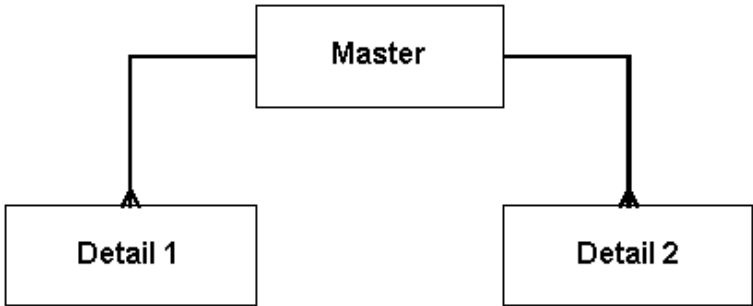
Description of "Figure 10-17 A simple fan trap schema"
