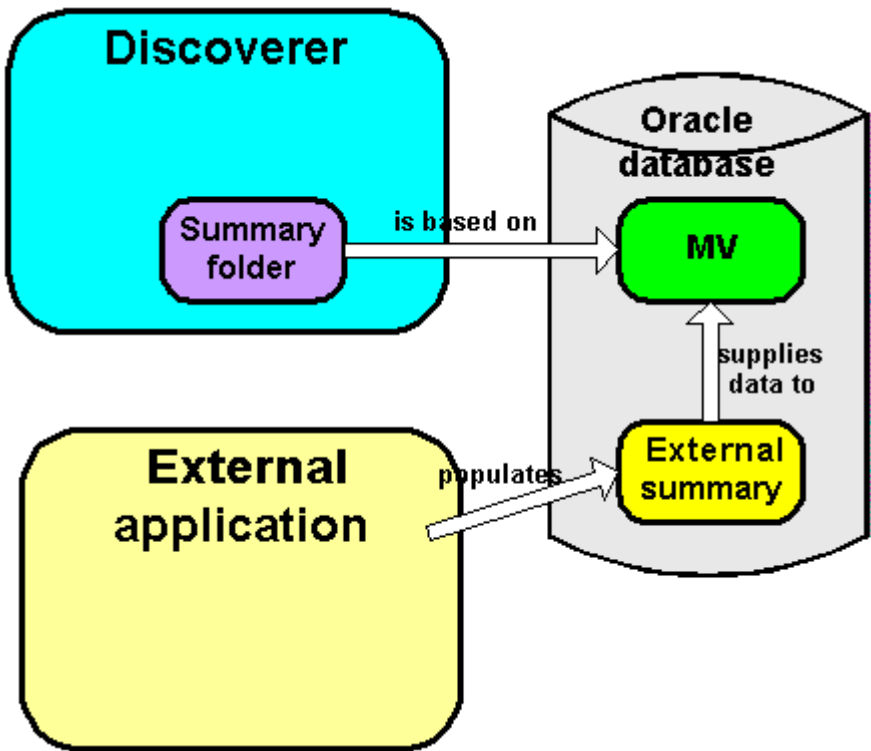
Description of "Figure 16-3 Discoverer using external summaries"
