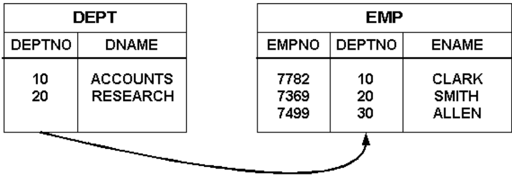
Description of "Figure 10-9 Scenario Two: An example of a schema where the rows returned depend on whether the master folder is included in the query"
