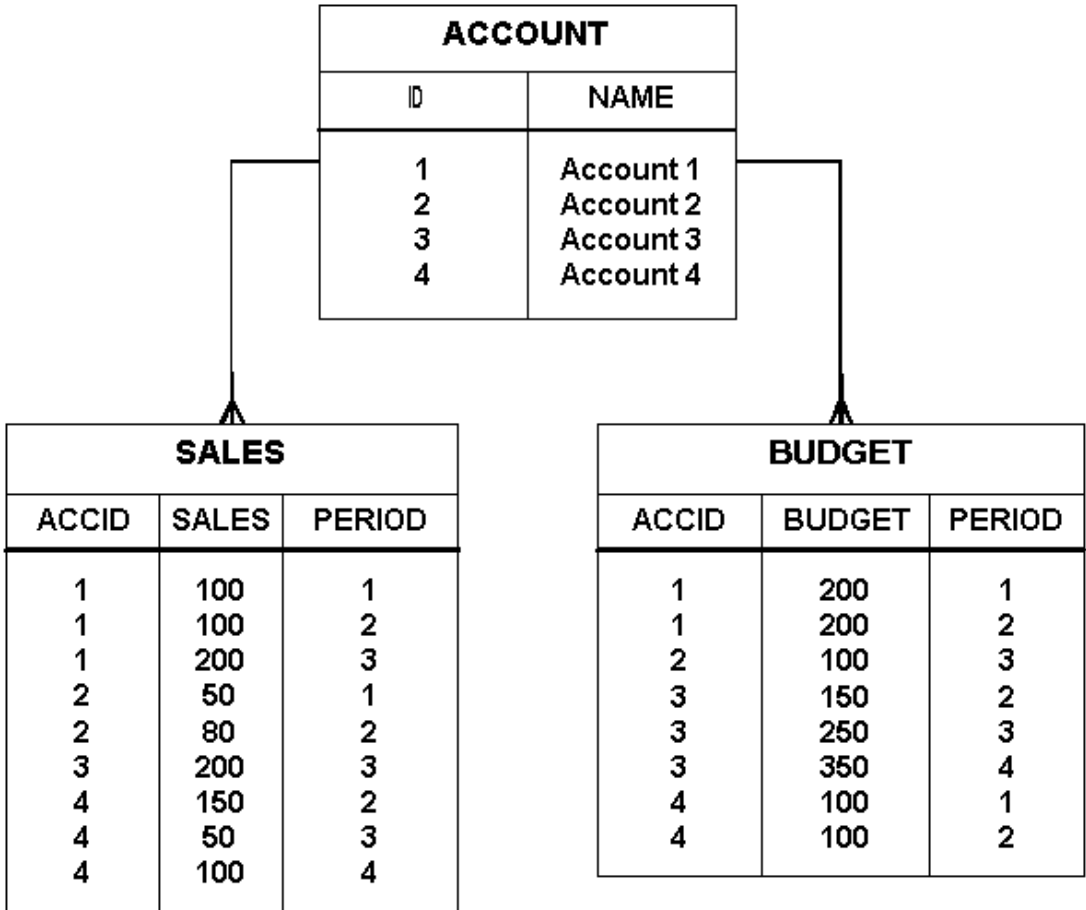
Description of "Figure 10-18 Example of a fan trap schema"
