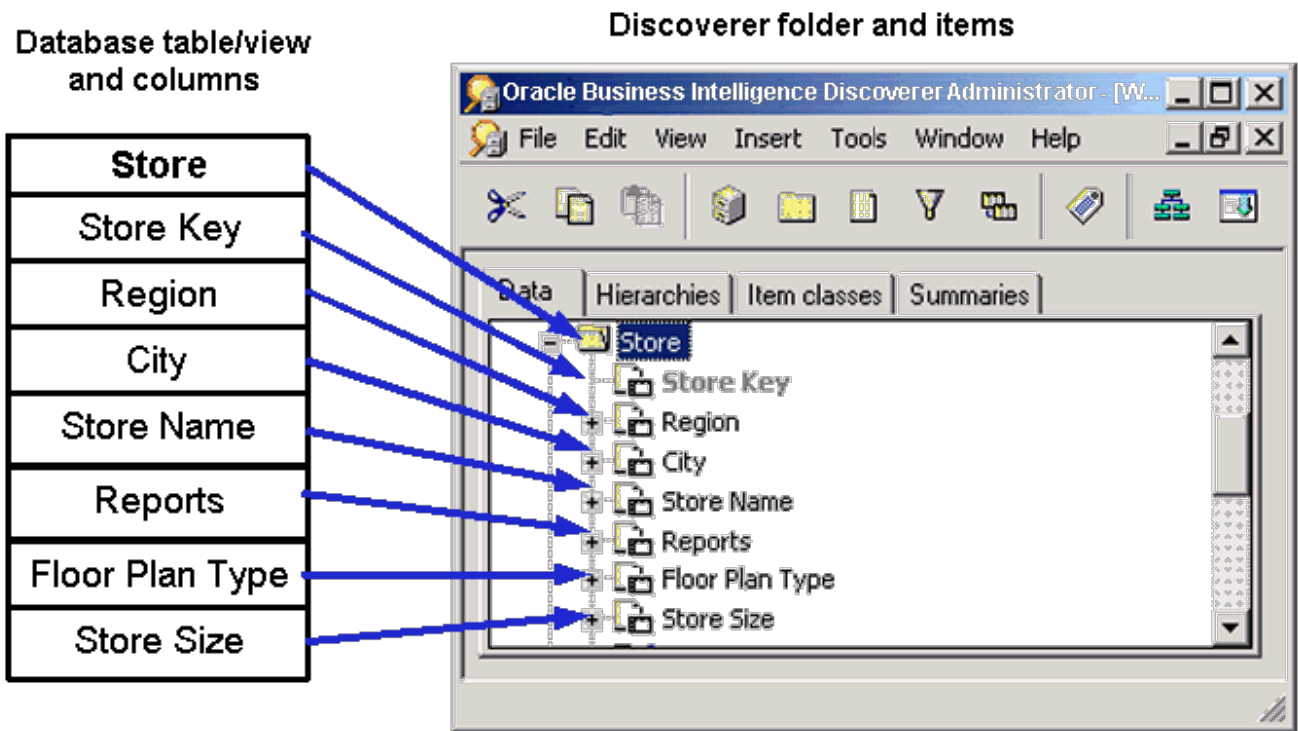
Description of "Figure 6-1 How Discoverer Administrator represents a table/view"
