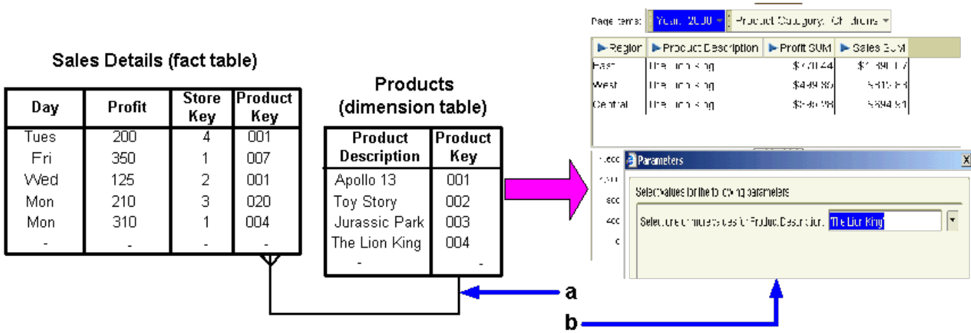
Description of "Figure 9-23 Part of a typical schema"
