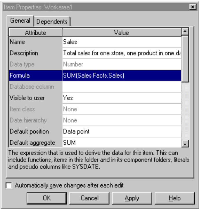
Description of "Figure 10-19 Example of an aggregate formula specified for an item in a complex folder"
