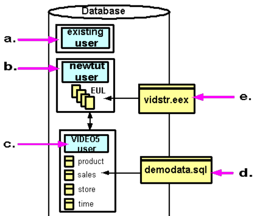
Description of "Figure 27-1 Events that can occur when you install the sample data"
