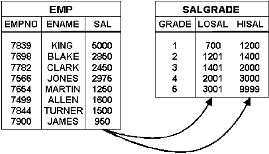
Description of "Figure 10-6 Example of two tables joined using a non-equi-join"
