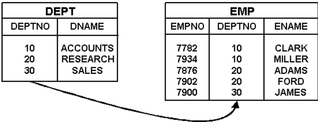
Description of "Figure 10-3 Example of two tables joined using a single item join"
