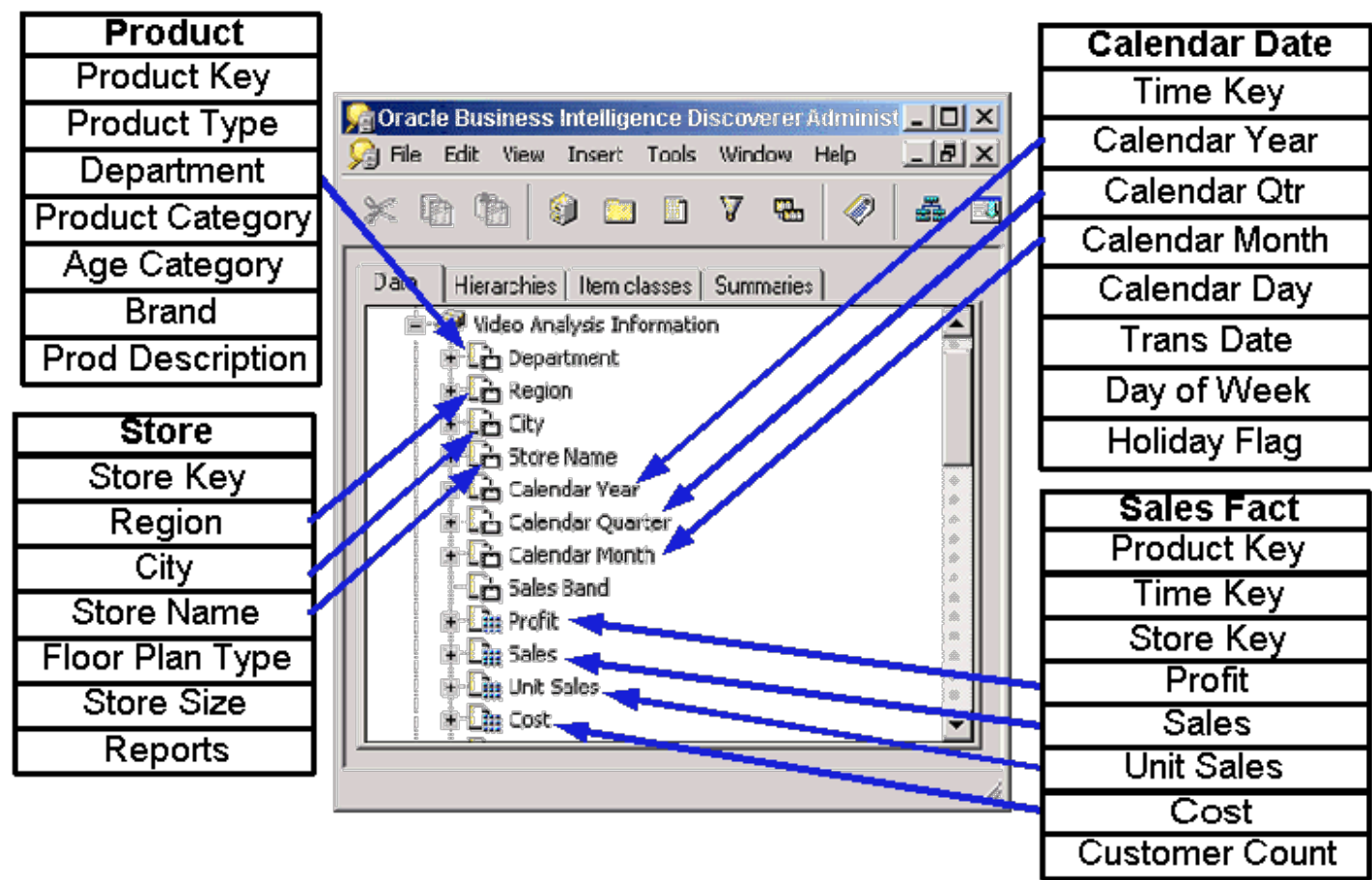
Description of "Figure 6-2 How a complex folder groups items from multiple source tables"
