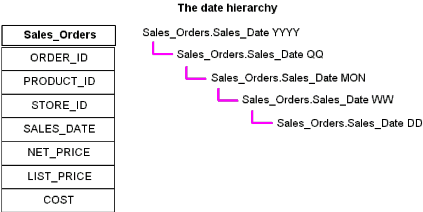
Description of "Figure 13-6 Sample date hierarchy - database perspective"
