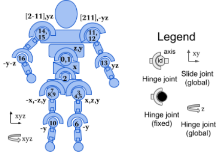
Fig. 2. Actuated joints of the MuJoCo humanoid: the 17 controllable hinge joints (3 abdomen, 3 per hip, 1 per knee, 2 per shoulder, 1 per elbow) that define the \mathbb{R}^{17} action space.
