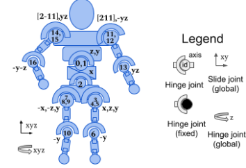
Fig. 2: Action space: 17 torque-controlled joints of the MuJoCo Humanoid.
