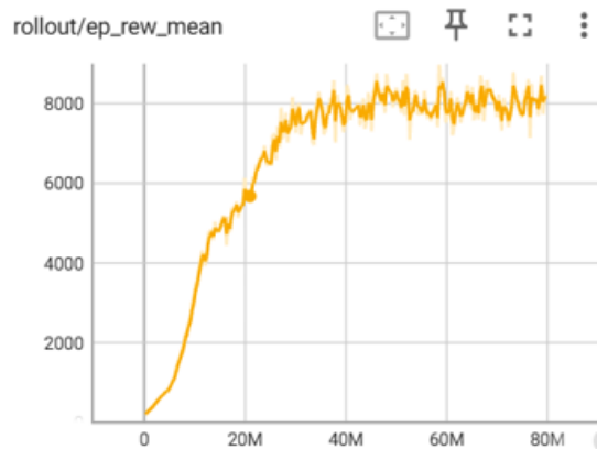
Fig. 6: S4 – Circuit with stairs: mean episode reward over 80M training steps. The best checkpoint at 64M and persistent plateau oscillations reflect the multi-objective complexity of the combined task.
