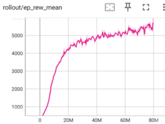
Fig. 5: S3 – Circuit navigation (flat): mean episode reward over 80M training steps. The absence of a clear plateau and the best checkpoint at 80M suggest the policy had not fully converged.
