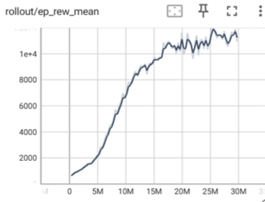
Fig. 4: S2 – Stair climbing: mean episode reward over 30M training steps. Rapid convergence with the best checkpoint at 29M steps reflects the effectiveness of climbing-specific reward shaping.
