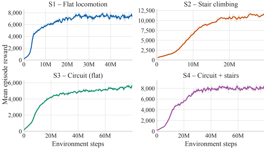
Fig. 3. Training curves for the four final runs: mean episode return per rollout batch in raw reward units (faded: raw; solid: EMA-smoothed). Reward scales are task-specific and not comparable across panels.
