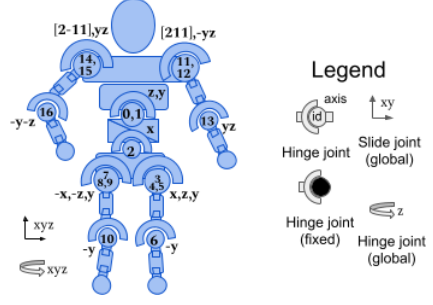
Fig. 2. Actuated joints of the MuJoCo humanoid: the 17 controllable hinge joints (3 abdomen, 3 per hip, 1 per knee, 2 per shoulder, 1 per elbow) that define the \mathbb{R}^{17} action space.
