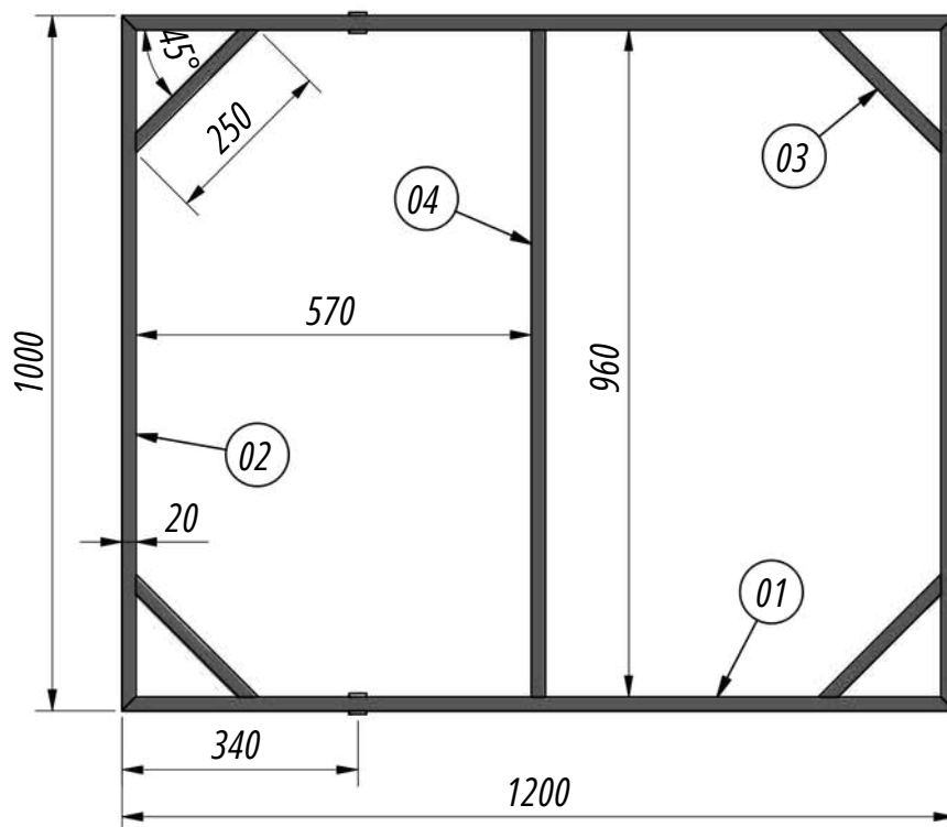
VISTA FRONTAL
