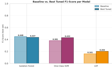
Fig. 5. Test-set F1-Score: default baseline vs. best hyperparameter configuration.
