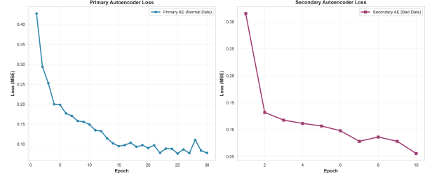
Fig. 6. Training loss (MSE) over epochs for the Primary and Secondary Autoencoders.
