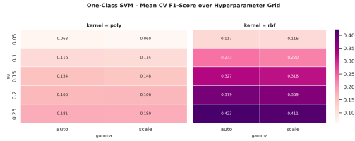
Fig. 5. OC-SVM mean CV F1-Score across nu and gamma configurations.
