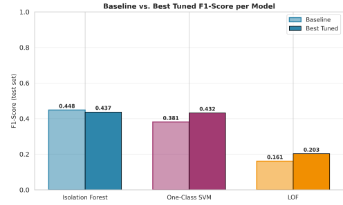
Fig. 7. Test-set F1-Score: default baseline vs. best hyperparameter configuration.
