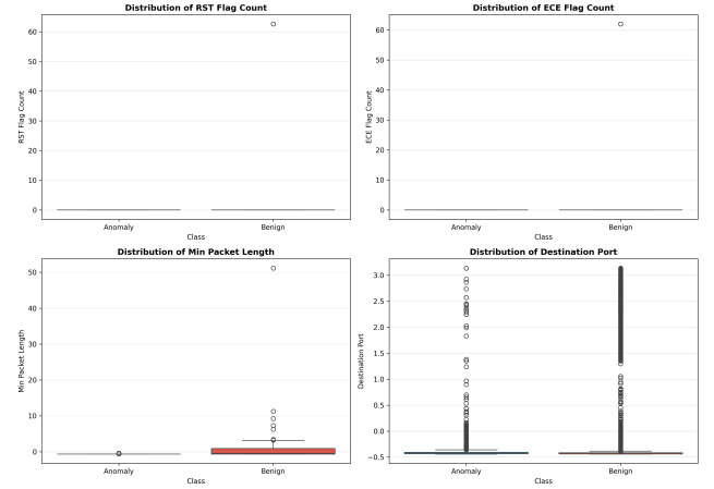
Fig. 2. Normalized distribution boxplots of four representative high-variance features grouped by traffic class (Benign vs Anomaly). This visual comparison highlights the complex, overlapping feature spaces that necessitate multi-dimensional unsupervised modeling.
