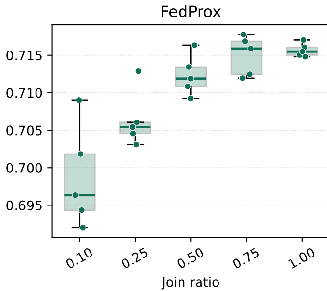
Best test accuracy by join ratio (n=5 per configuration)
